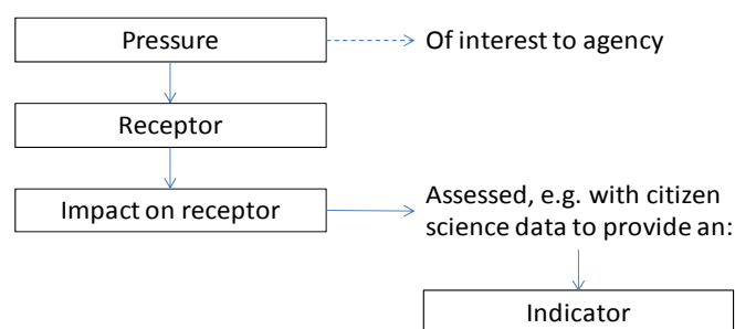
Fig. 2. Idealised role of citizen science in contributing to an official indicator of an environmental pressure. For any indicator each of the steps should be empirically quantified and there should be a unique link between the pressure and the indicator (or such a link should be determinable once confounded factors have been taken into account statistically).
